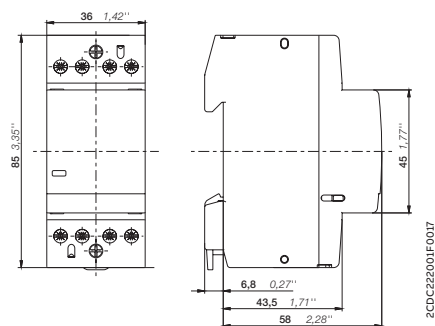
ESB25..N Abmessungen mm, Zoll
