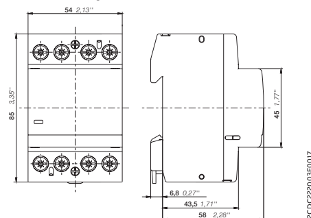
ESB40..N Abmessungen mm, Zoll
