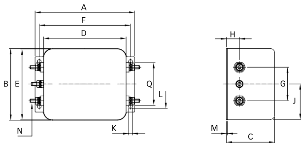
Connection style -08, 30 A types
